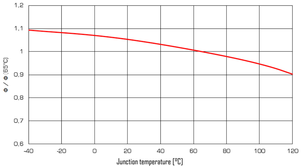
LUMINOUS FLUX vs. TEMPERATURE
